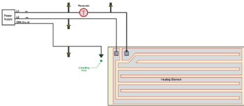
Figure 1: Standard Wiring Diagram
